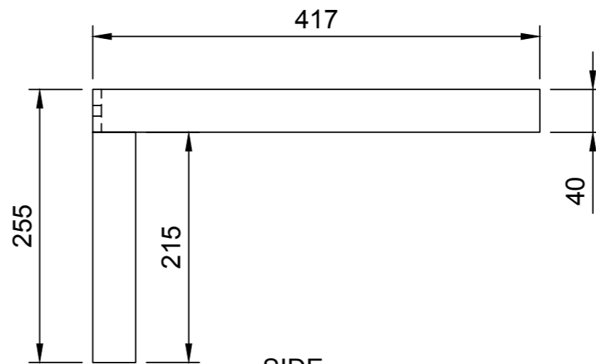
SIDE
