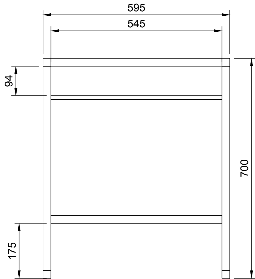
FRONT
