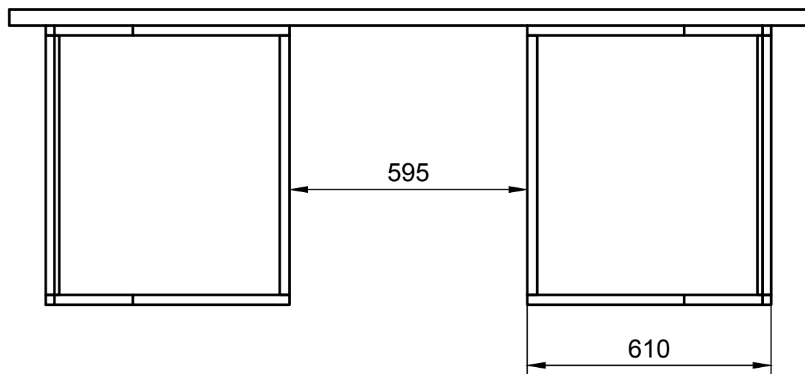
FRONT
